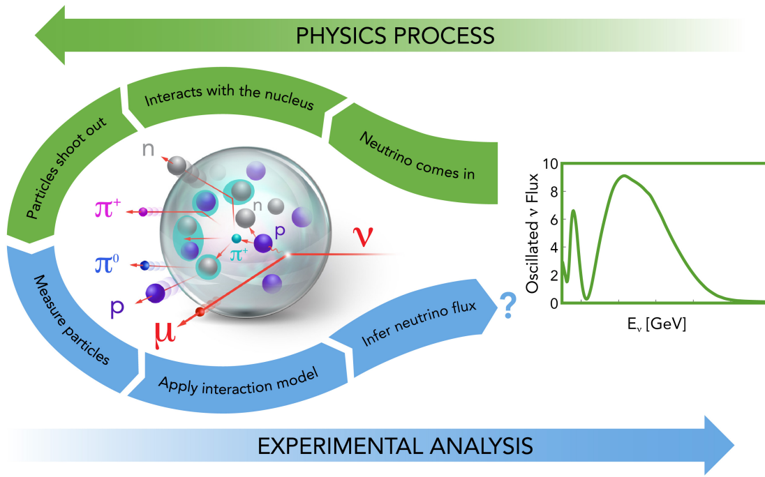
Fig. 1: Neutrino oscillations and energy spectra measurements | (Left) Neutrino energy spectra reconstruction depends on our ability to model the interaction of neutrinos with atomic nuclei and the propagation of particles through the atomic nucleus. This flow chart shows the process, starting with an oscillated far-detector incident-energy spectrum (green), differentiating the physical neutrino interactions (green arrows) from the experimental analysis (blue arrows), and ending up with an inferred incident-energy spectrum that hopefully matches the actual one.
