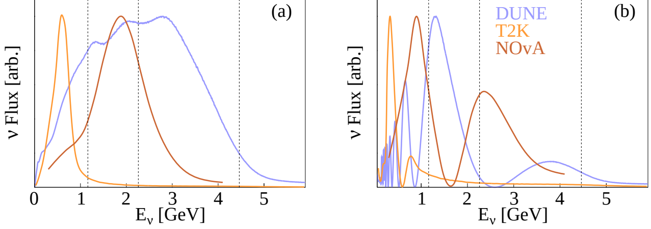
Fig. Extended Data Fig. 1: The expected energy distribution of different \nu_\mu beams, (left) before oscillation at the near detector and (right) after oscillation at the far detector [59, 60]. The vertical lines show the three electron beam energies of this measurement. The NO \nu A far-detector beam flux is calculated using the near detector flux and the neutrino oscillation parameters from the Particle Data Group.
